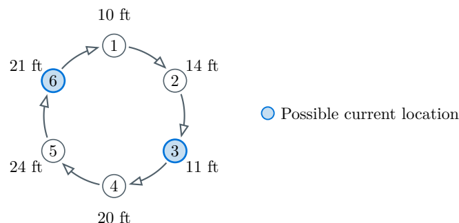
Figure 2: Example of checkpoints (10, 14, 11, 20, 24, 21) with readings (100, 104, 101) .
